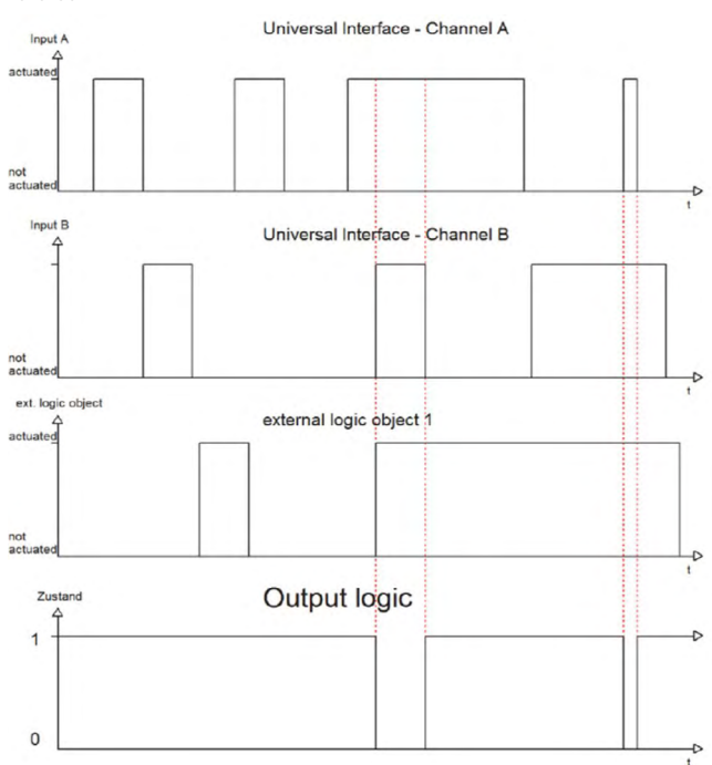
Figure 29: Logic output
